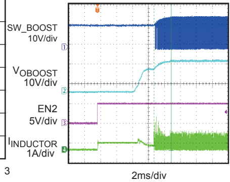
Boost Regulator EN2 Start Up
