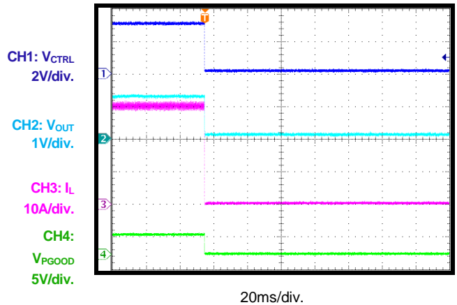
Power-Off through CTRL, CCM, I_{OUT} = 30A , Single-Phase
