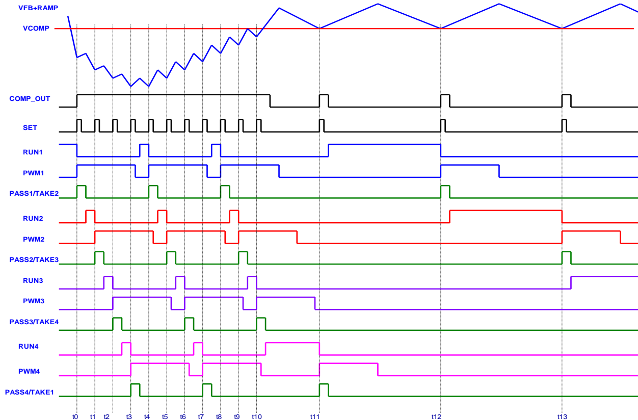
Figure 3: Multi-Phase Interleaved Operation (Steady State)
