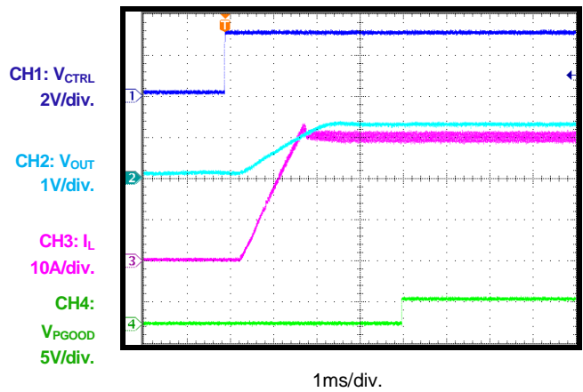
Power-On through CTRL, DCM, I_{OUT} = 30A , Single-Phase
