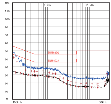
EMI Performance 230 N Line
