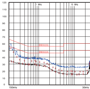
EMI Performance 230 L Line
