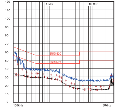
EMI Performance 115 L Line
