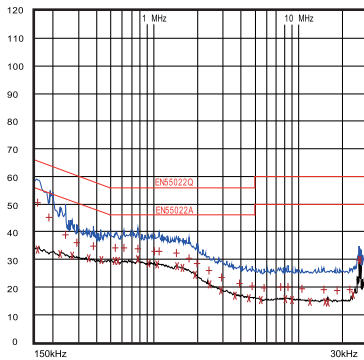
EMI Performance 115 N Line
