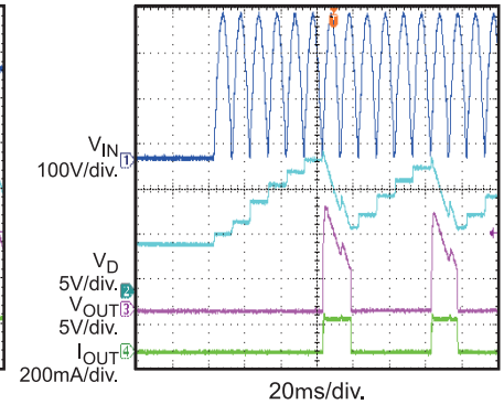
Over Load Protection Entry
