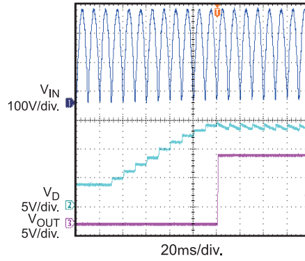
Thermal Shutdown Protection Recovery V_{IN} = 230V_{AC}
