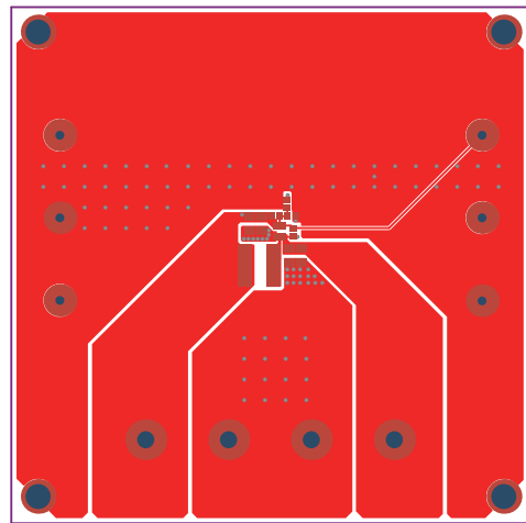
Figure 3: Top Layer
