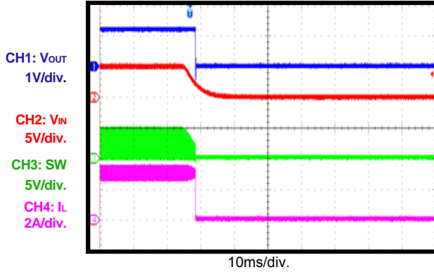
Vin Power Off with 3A load
