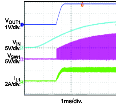
Startup through Input Voltage (CH1)
