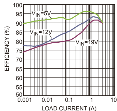
Efficiency vs. Load Current V OUT =3.3V, L=4.7µH
