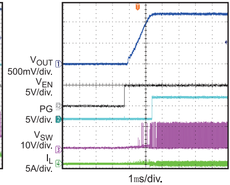
Start-Up through EN Forced PWM, I_{OUT}=0A
