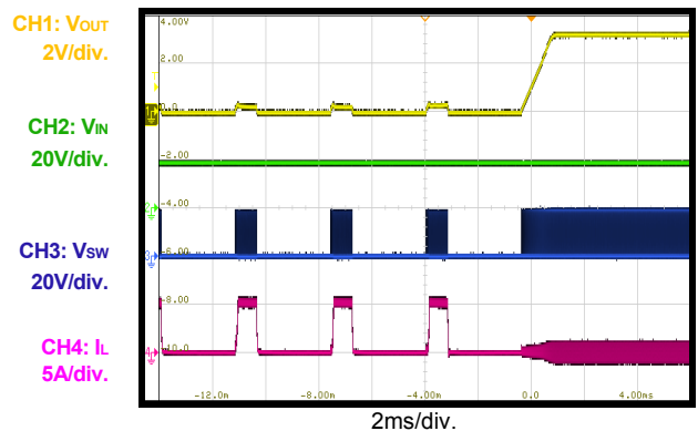
Short-Circuit recovery
