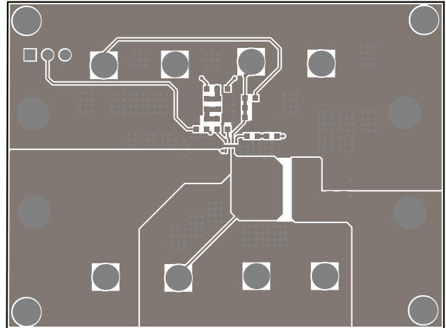
Figure 2: Top Layer
