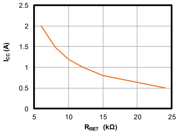
I_{CC} vs. R_{ISET}
