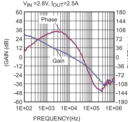
Bode Plot
