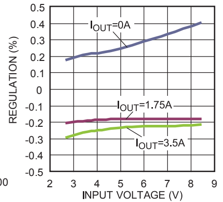
Line Regulation (PSM)
