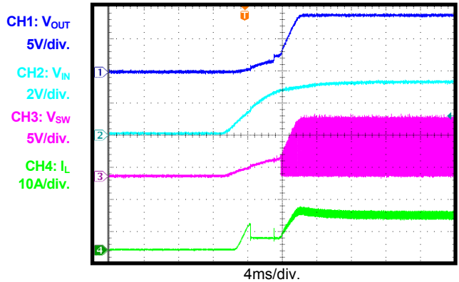
V_{IN} Start-Up I_{OUT} = 3.5A
