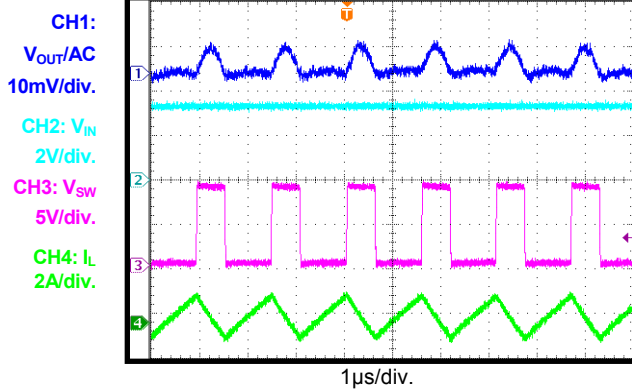
Steady State I_{OUT} = 0A , FCCM
