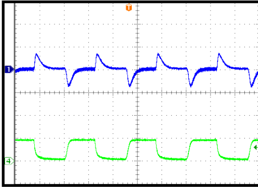
Load Transient
