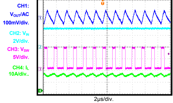
Steady State I_{OUT} = 3.5A
