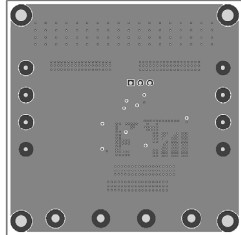
Figure 4—Inner Layer 2
