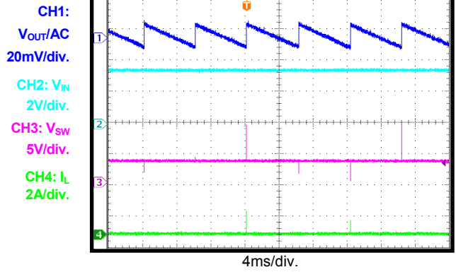
Steady State I_{OUT} = 0A , PSM
