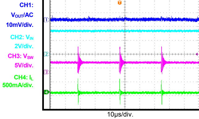
Steady State I_{OUT} = 0A , USM
