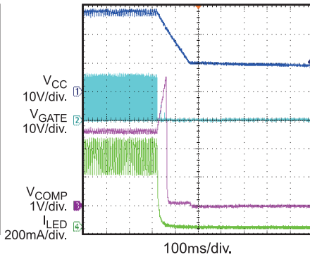
V_{IN} Shut-Down
