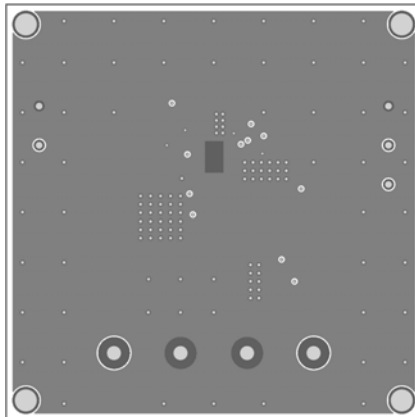
Figure3 – Inner Layer 1
