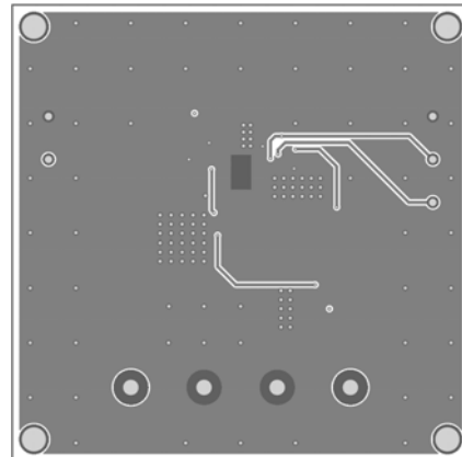
Figure 4 – Inner Layer 2
