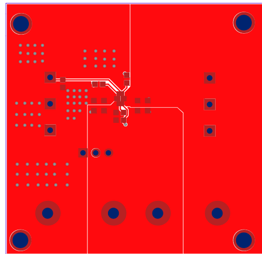
Figure 2: Top Layer
