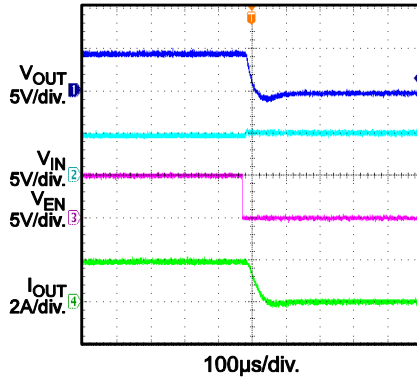
Shutdown through Enable I_{LOAD}=2A
