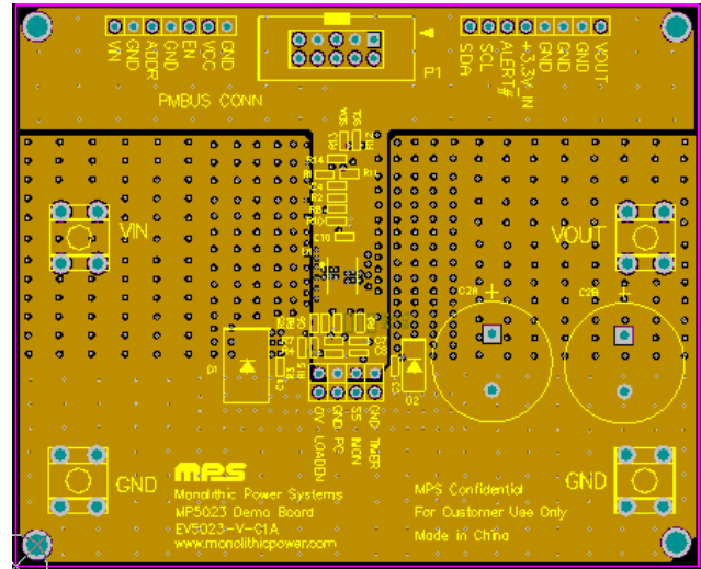
Figure 2—Inner Layer1
