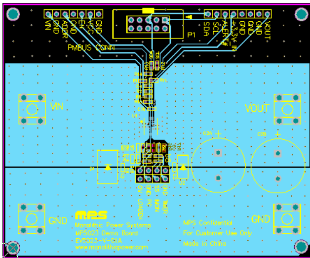
Figure 3—Inner Layer2
