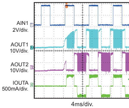
Power Ramp Up-Half Step V_{IN}=15V
