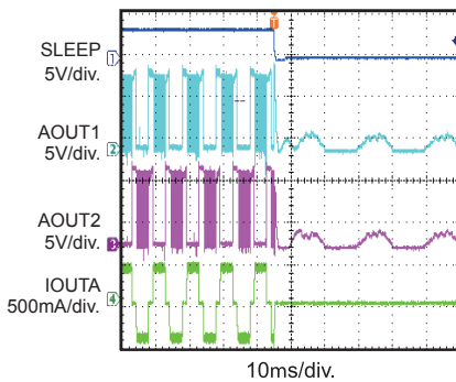
Sleep Entry-Half Step V_{IN}=9V
