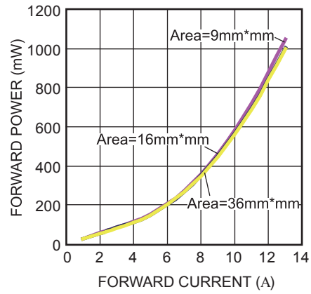
Forward Power Dissipation
