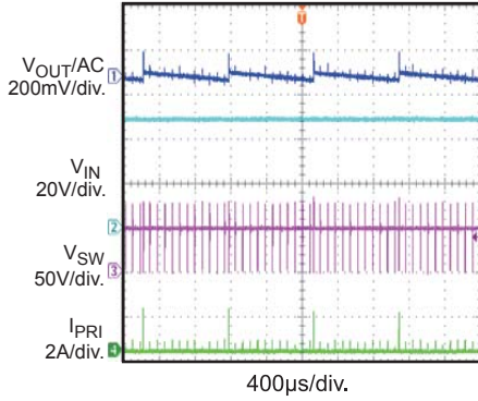
Steady State I_{OUT} = 10mA
