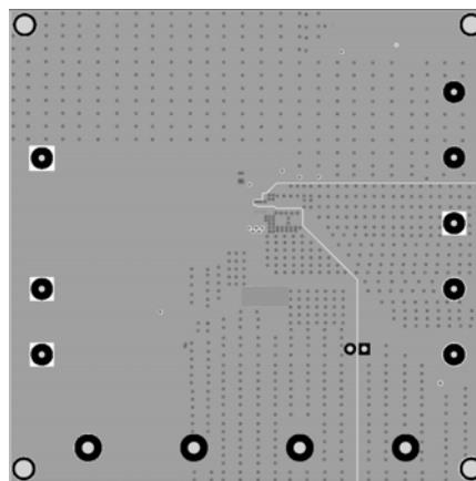
Figure 5: Bottom Layer
