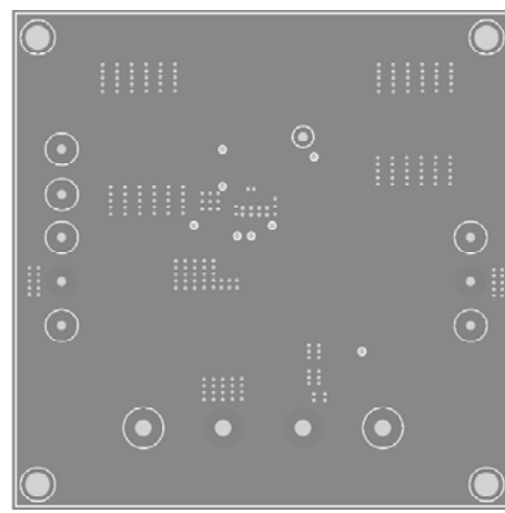
Figure 4—Inner2 Layer
