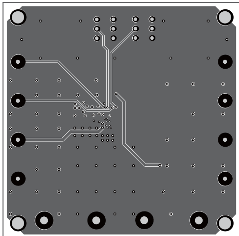
Figure 3—Inner Layer 2
