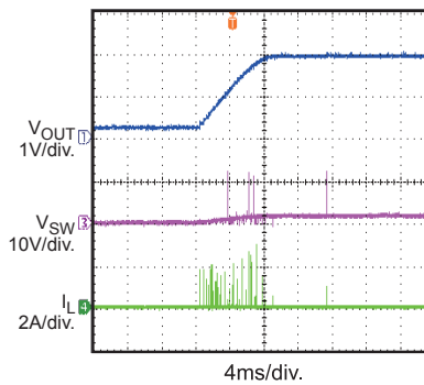
Thermal Recovery I_{OUT}=0A
