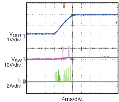
Thermal Recovery I_{OUT}=0A
