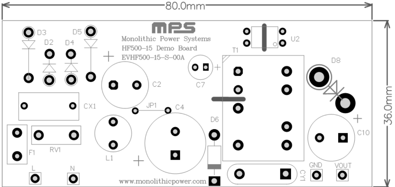
Figure 2: Top Layer
