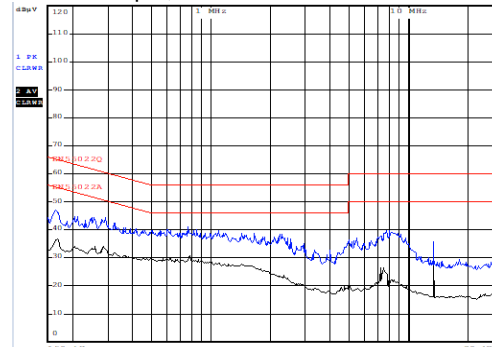
Conducted EMI
