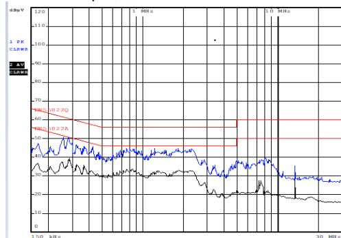
Conducted EMI
