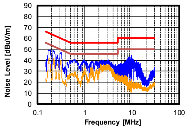
Conducted EMI
