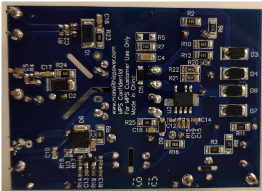
BOTTOM VIEW
