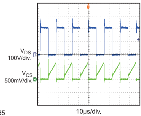
Voltage Stress
