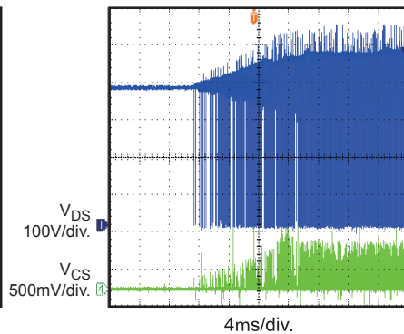
Soft Start
