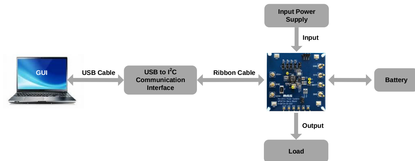
Figure 1: EVKT-MP2672A Evaluation Kit Set-Up
