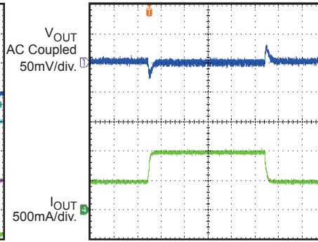
Transient Response
