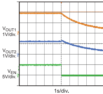
EN Down without Load I_{OUT1} = I_{OUT2} = 0A
