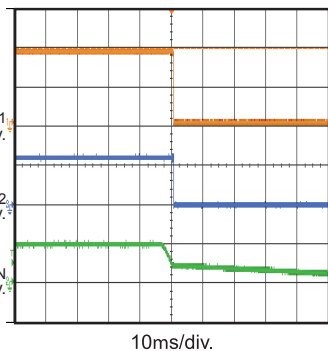
V_{IN} Power Down with 2A Load I_{OUT1} = I_{OUT2} = 2A
