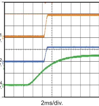
V_{IN} Power Up with 2A Load I_{OUT1} = I_{OUT2} = 2A
