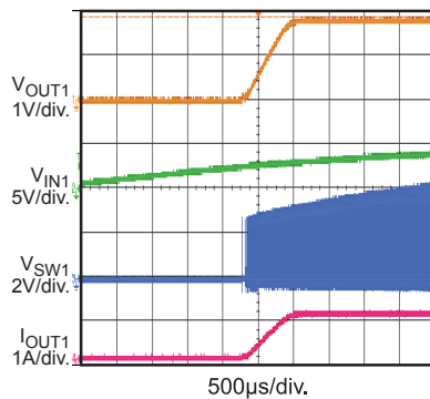
VIN Power On with 1A Load I_{OUT1} = 1A , I_{OUT2} = 0A
