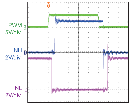
Generated INH and INL from PWM
