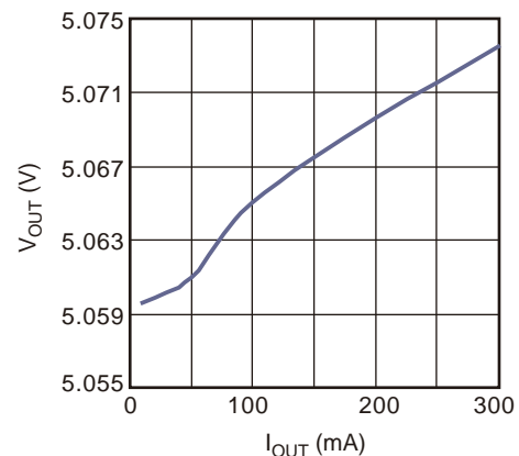
V OUT vs. I OUT V IN =6V
