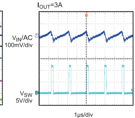
Input Ripple Voltage
