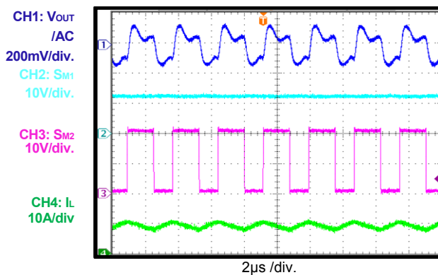
Steady state , V_{OUT}=20V Load=5A
