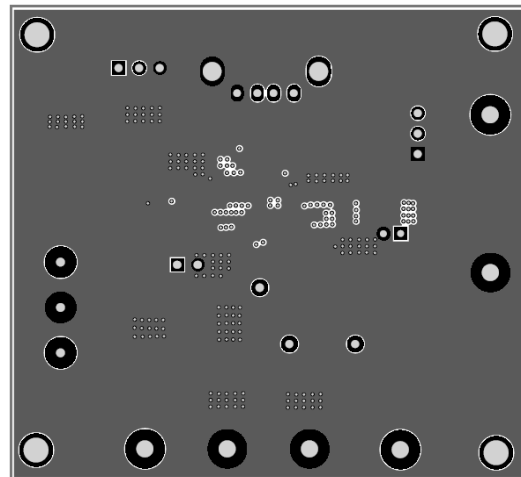
Figure 4—Mid 2 Layer
