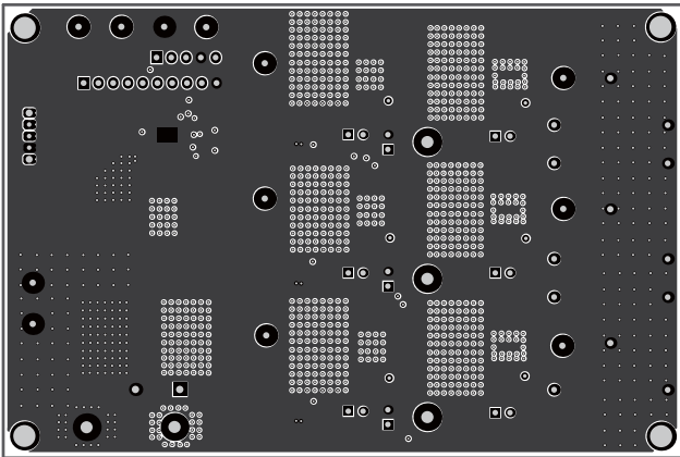
Figure 3: Inner1
