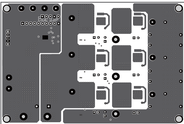
Figure 5: Bottom
