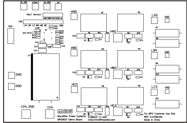
Figure 2: Top Silk
