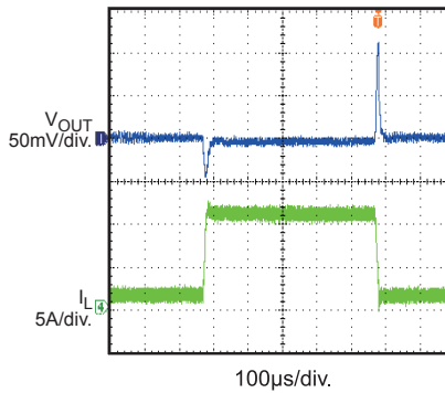
Transient Response I_{OUT}=1.2A\sim 10.8A @ 1.6A/\mu S , F_s=600kHz , C_{OUT}=4x22\mu F
