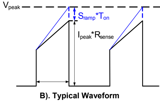
Figure 12: Peak Current Comparator
