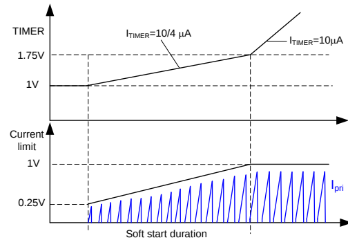
Figure 6: Soft Start
