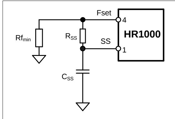
Figure 8: Soft-Start Block
