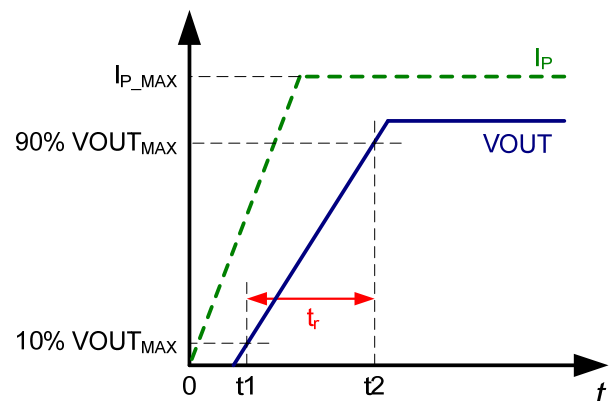
Figure 6: Rise Time ( t_r )
