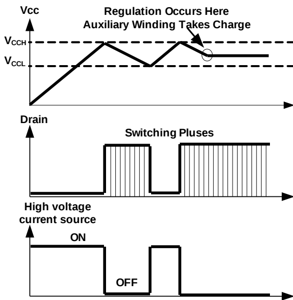
Figure 2: VCC Under-Voltage Lockout
