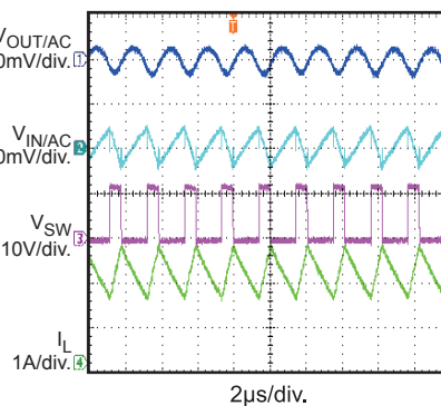
Input/Output Ripple I_{OUT} = 2A
