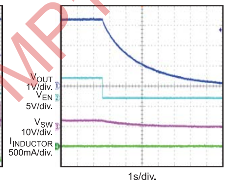
Shutdown through Enable
