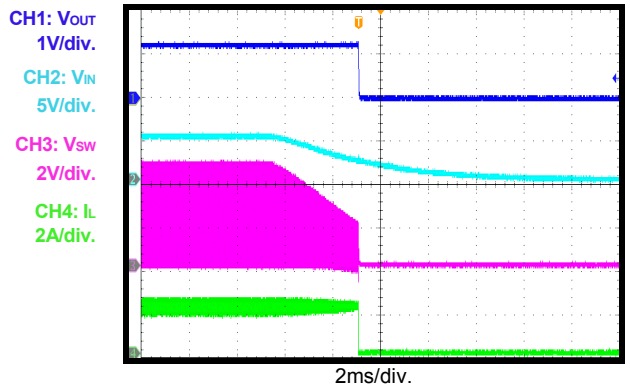
V_{IN} Shutdown
