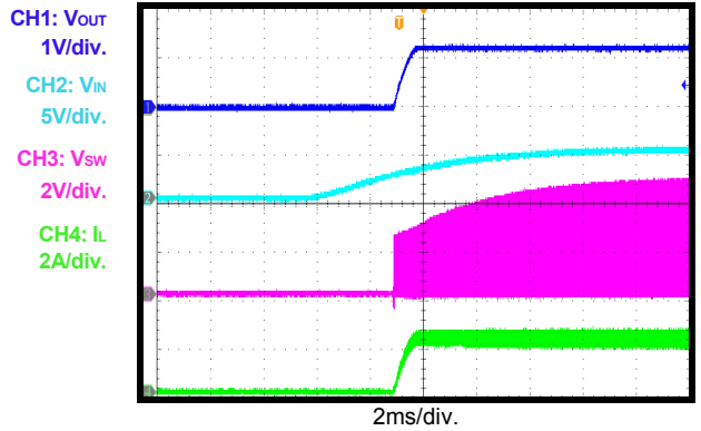
V_{IN} Power-Up
