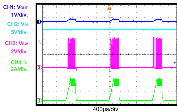
Short-Circuit State
