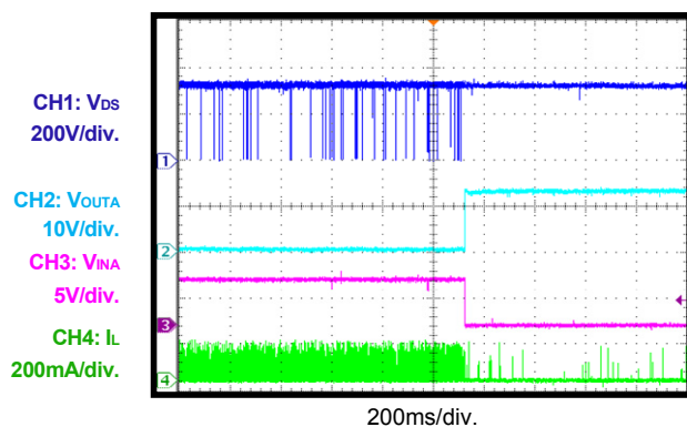
Relay 2 Turn-Off
