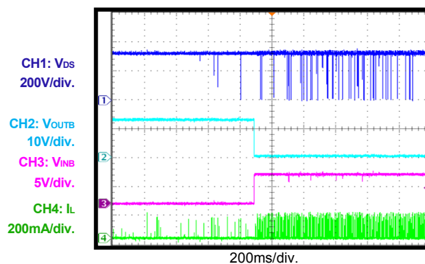
Relay 2 Turn-On
