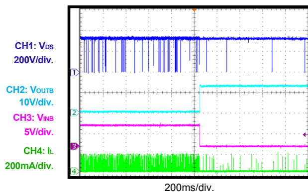
Relay 2 Turn-Off
