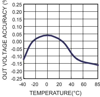
Out Voltage Accuracy vs. Temperature
