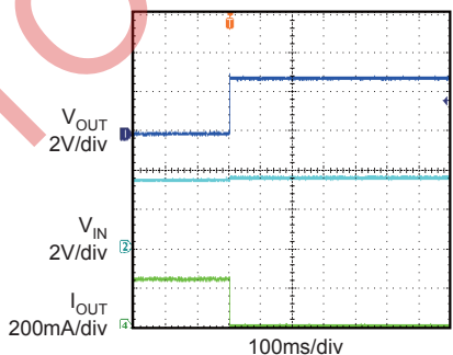
Over Current Protection Recovery
